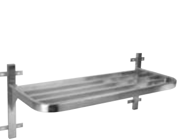
SINGLE WALL MOUNTED PRS0900 900 X 400 X 400MM
